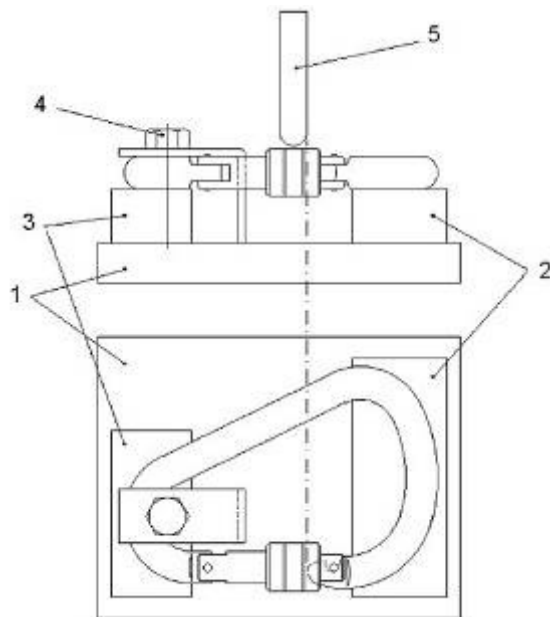
Figure 2 Locked-gate side-strength testing
